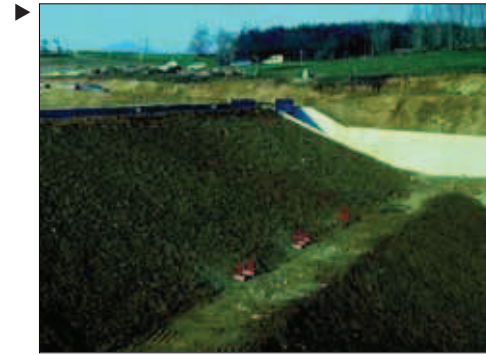
13 - Topsoil covering the downstream face of the same dam. Note the berm. (text p. 76).
