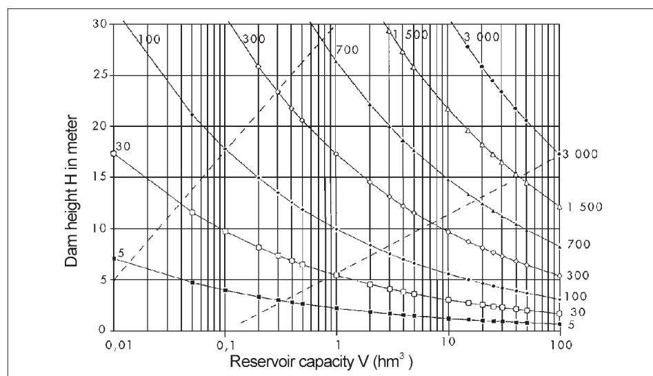
Fig. 1 - Height I Reservoir Capacity Relationship with values of H^2\sqrt{V} (V in hm 3 , H in metres)
