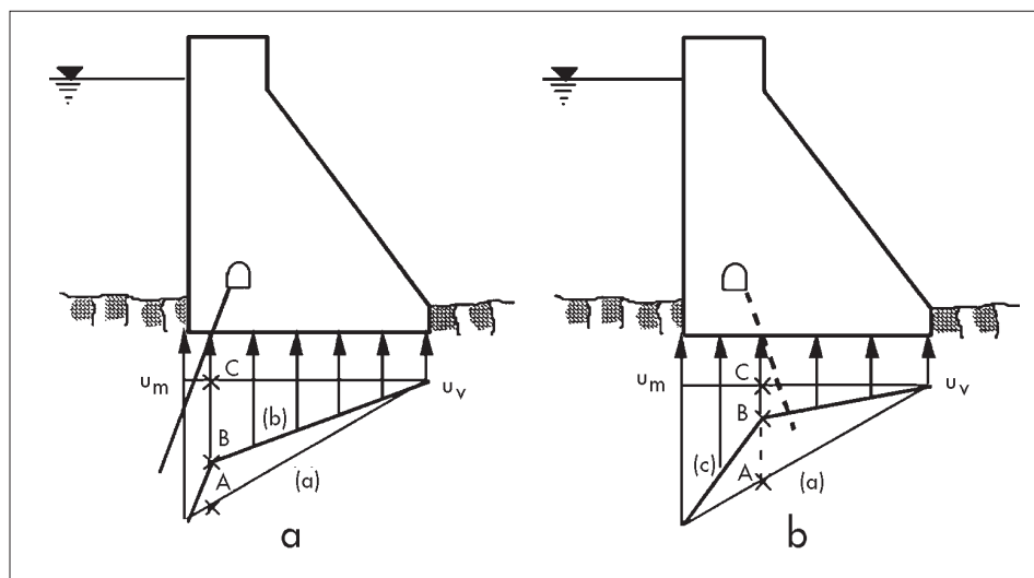
Fig. 2 - Indicative diagram of uplift:
