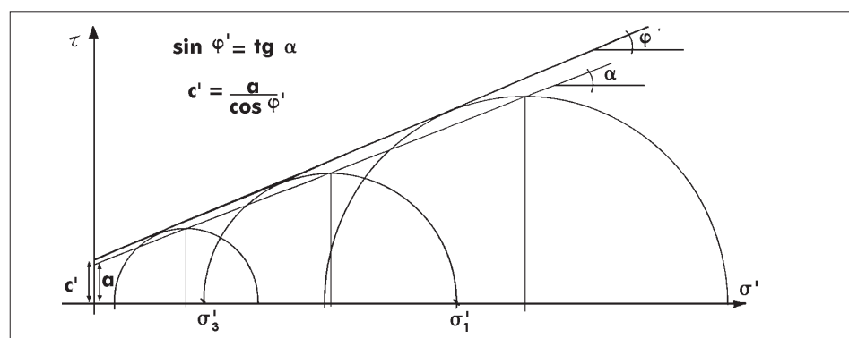
Fig. 5 - Relation between Mohr-Coulomb failure criteria and maximum shear strength
