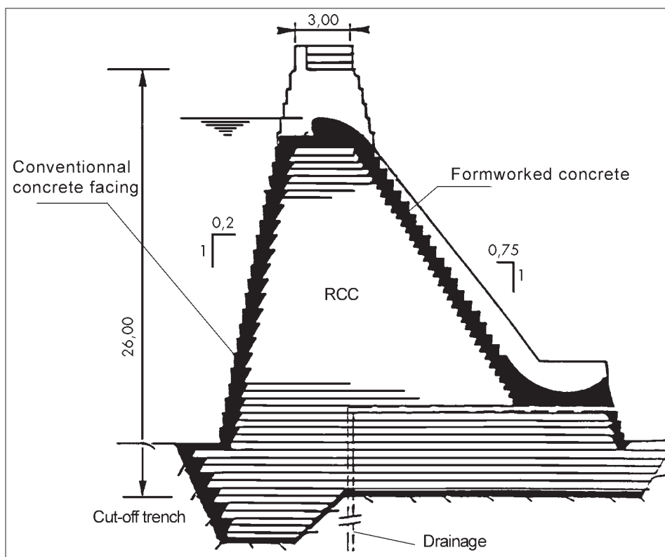
Fig. 5 - Typical cross-section of EL KOREIMA dam
